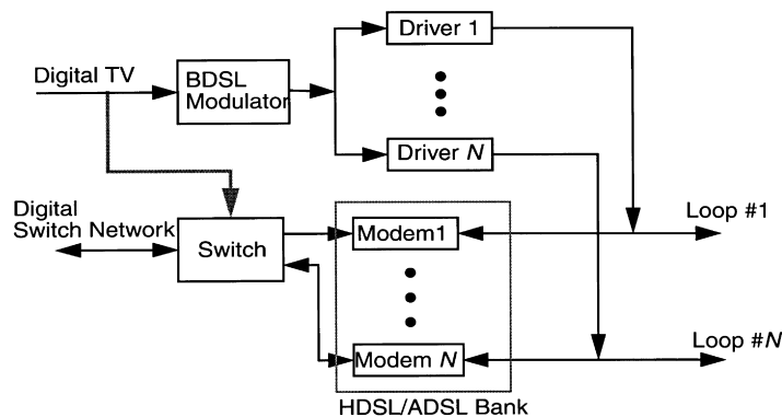
Fig. 2. The architecture of the central office modem bank of the BDSL systems.
