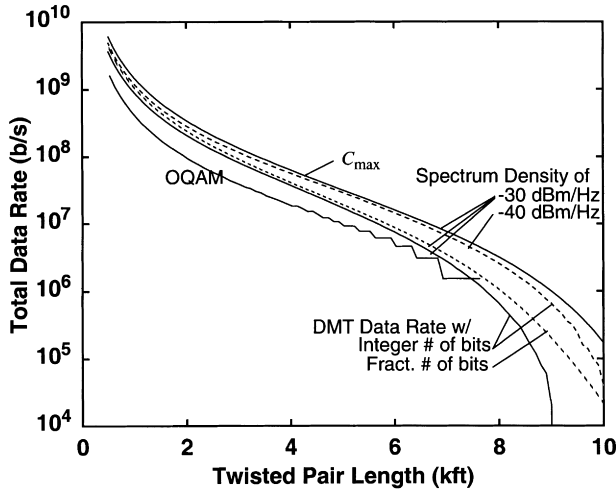
Fig. 5. Channel capacity and DMT maximum data rate of BDSL systems as a function of twisted-pair length. The maximum data rate of OQAM scheme is also shown for comparison.
