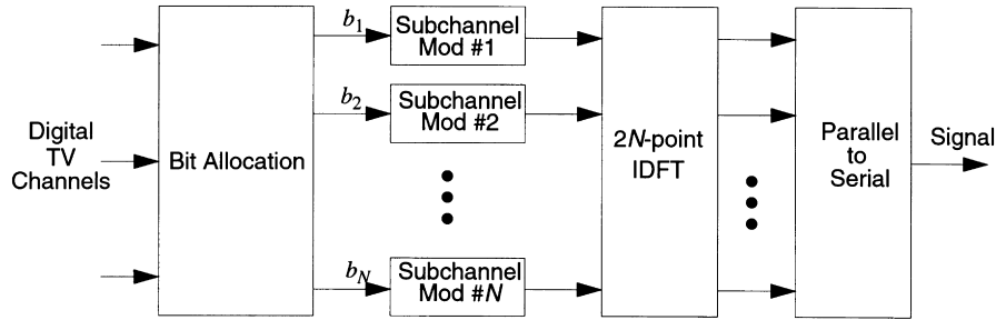
Fig. 3. The DMT transmitter of BDSL.
