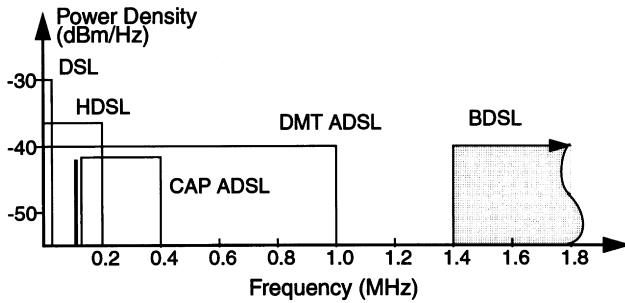
Fig. 1. Spectrum density of various digital subscriber line systems.
