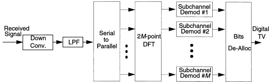
Fig. 4. The DMT receiver of BDSL.
